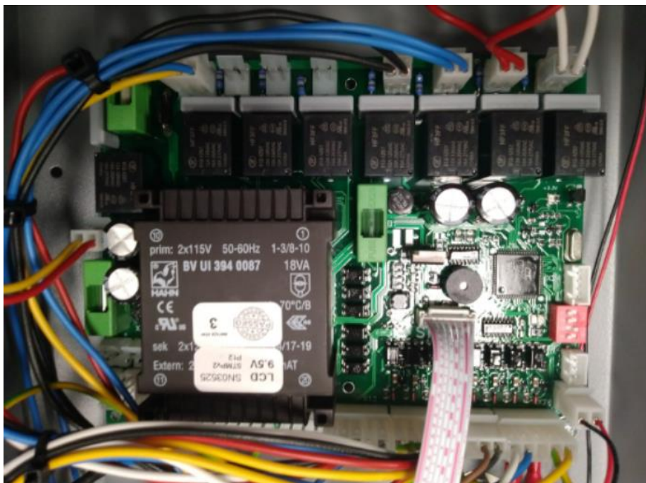
Main printed board (front)
