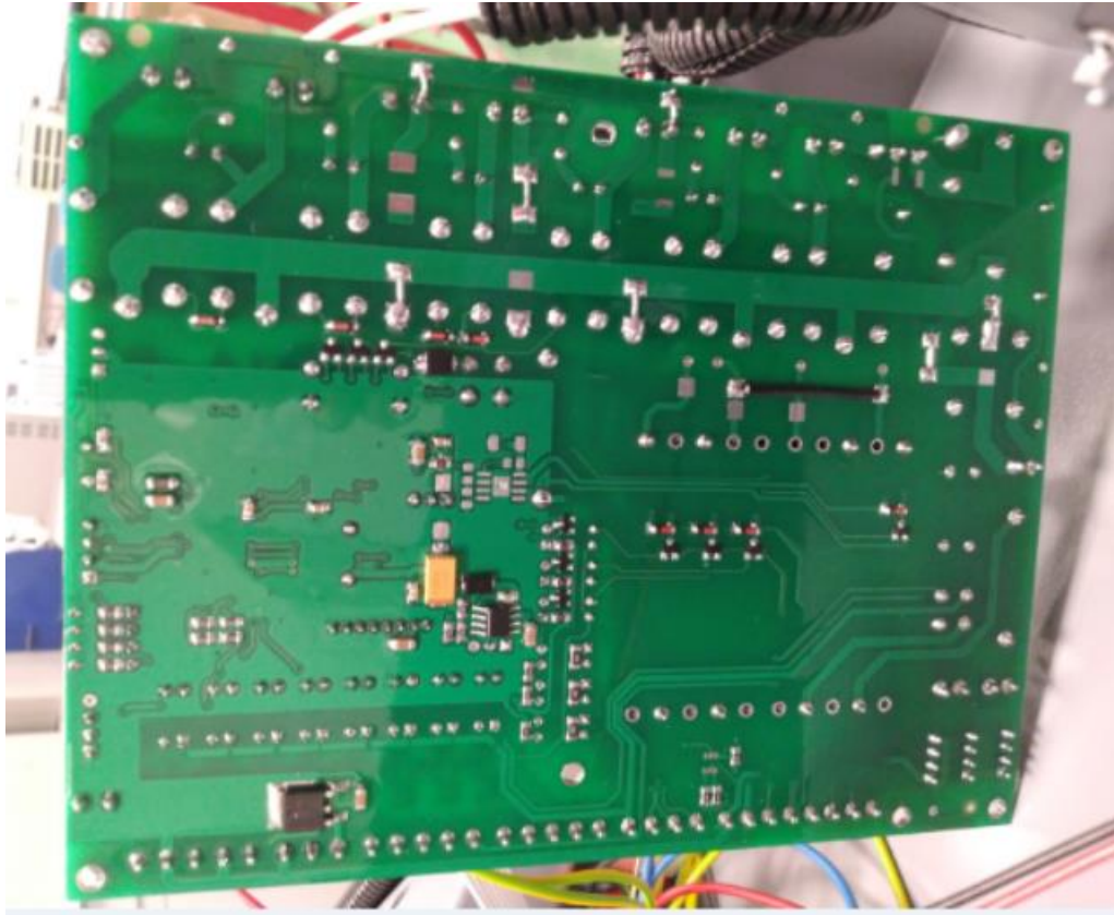
Main printed board (rear)
