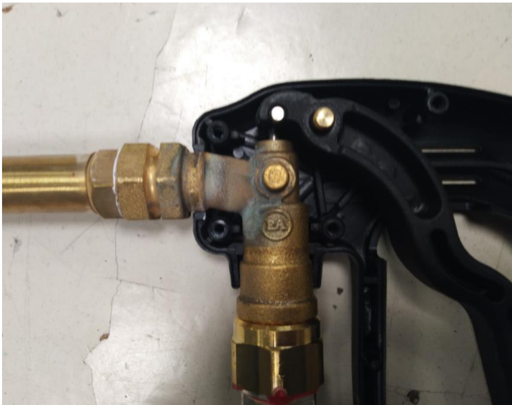
Detail of trigger gun mechanism
