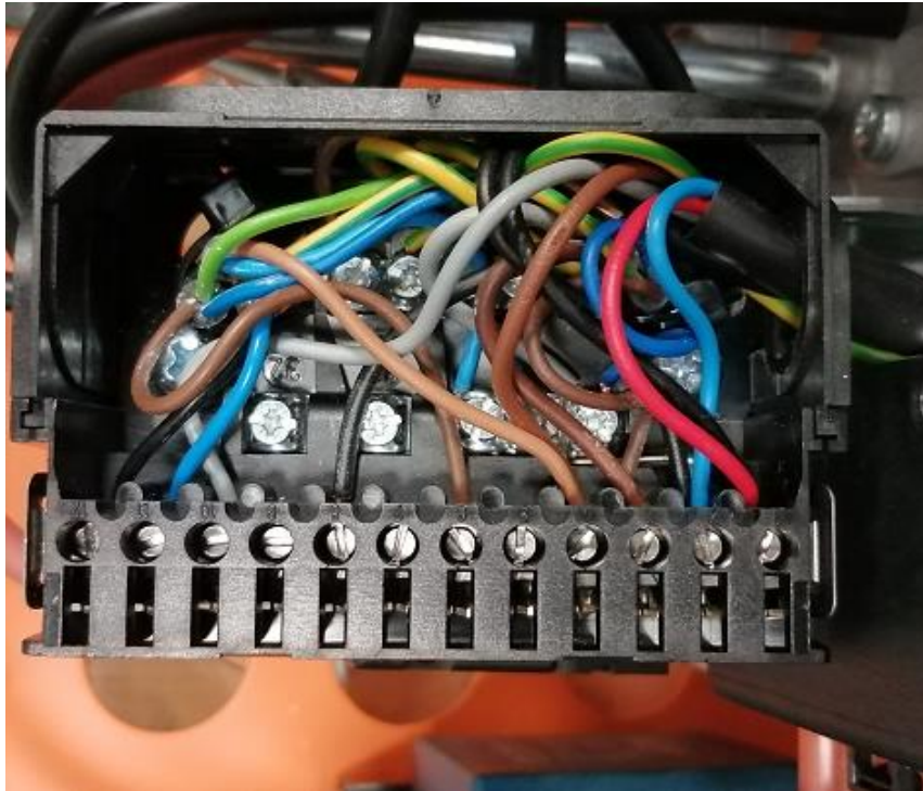
Ignition board unit connection
