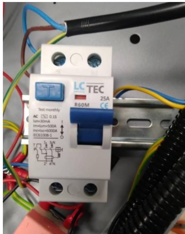
Residual current device
