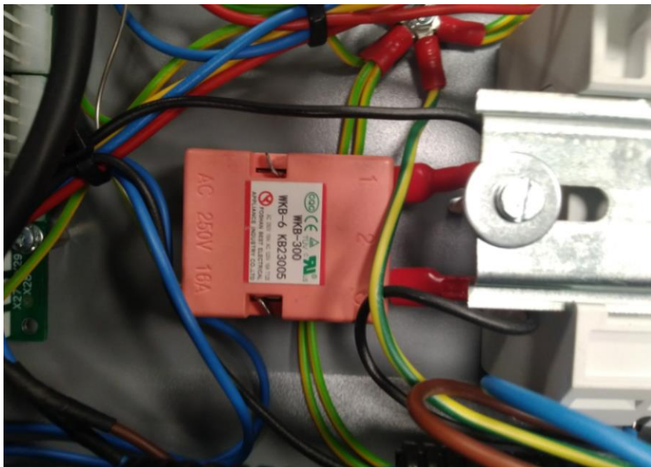
Capillary self resetting thermal cut-out
