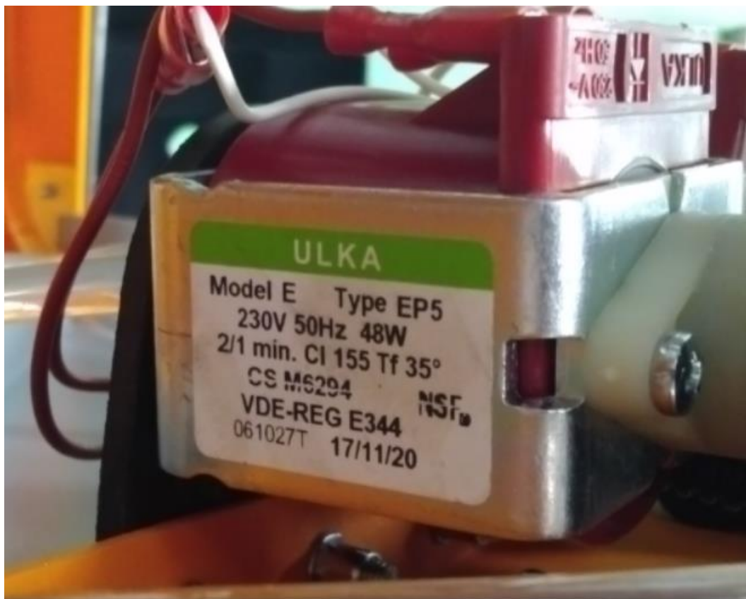
Vibrating pump markings
