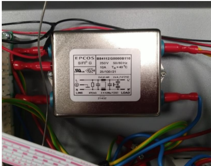
Main radio interference filter
